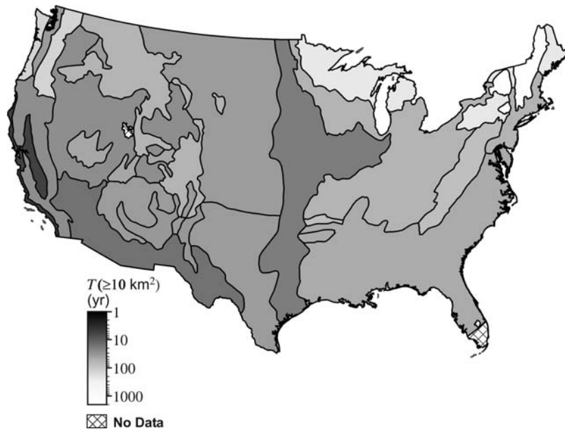
Fig. 3. Spatial mapping of wildfire recurrence intervals for the conterminous USA by ecoregion division (figure after Malamud et al. 2005). Based on a power-law frequency–area relationship from empirical data for the period 1970–2000 (see Fig. 2), recurrence intervals show how many years on average a wildfire of 10 km 2 or larger would be expected in spatial areas of 1000 km 2 within each ecoregion division. The legend colours go from black (small recurrence intervals) to white (large recurrence intervals), representing ‘high’ to ‘low’ hazard, with the legend scale in years increasing logarithmically.
